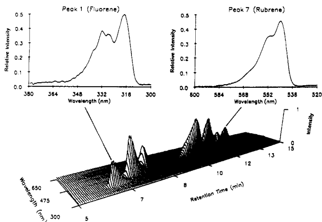
Figure 14. Chromatogram of a seven-component mixture of polycyclic aromatic hydrocarbons (reprinted from ref 95, copyright 1990 American Chemical Society).
