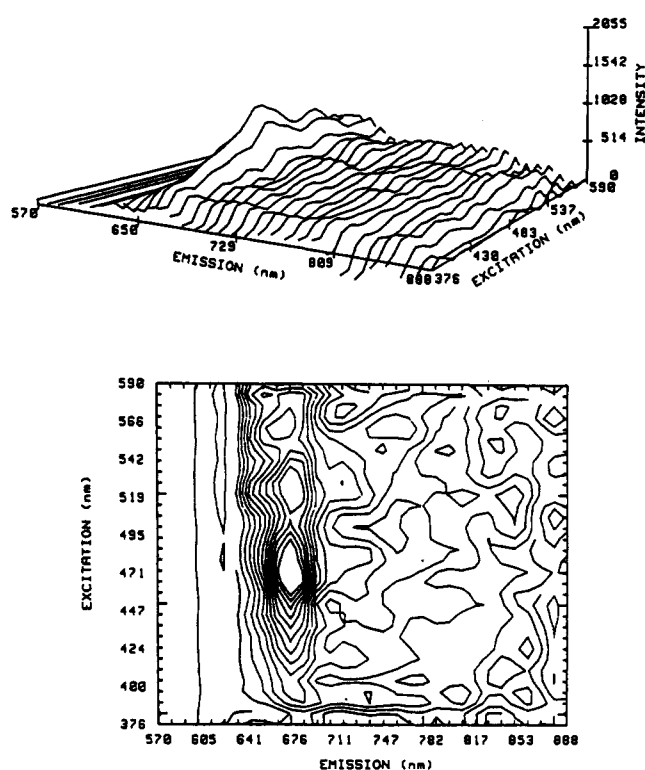
Figure 10. EEM of algae from the Gulf of Mexico (reprinted from ref 17, copyright 1987 Marcel Dekker Inc.).
