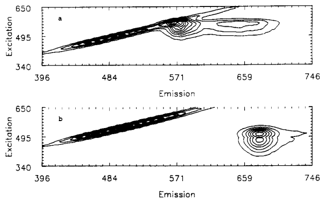
Figure 12. Contour plots representing (a) blue-green and (b) green algae.
